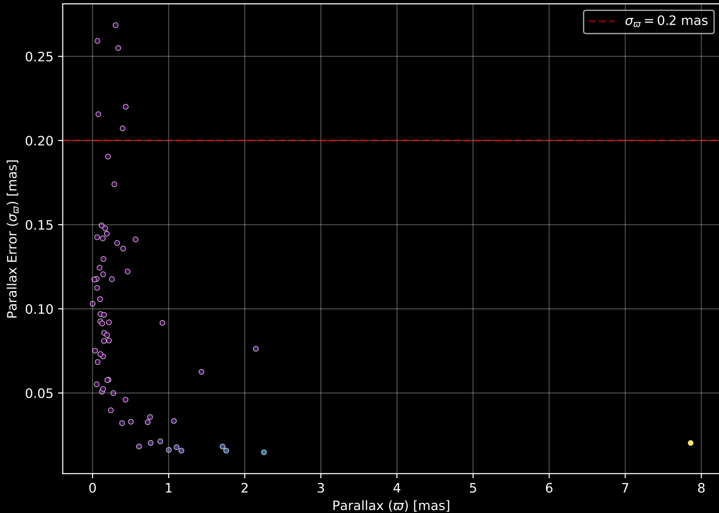
APOGEE DR17 Field: [359+01] Parallax Quality (n= 65)
