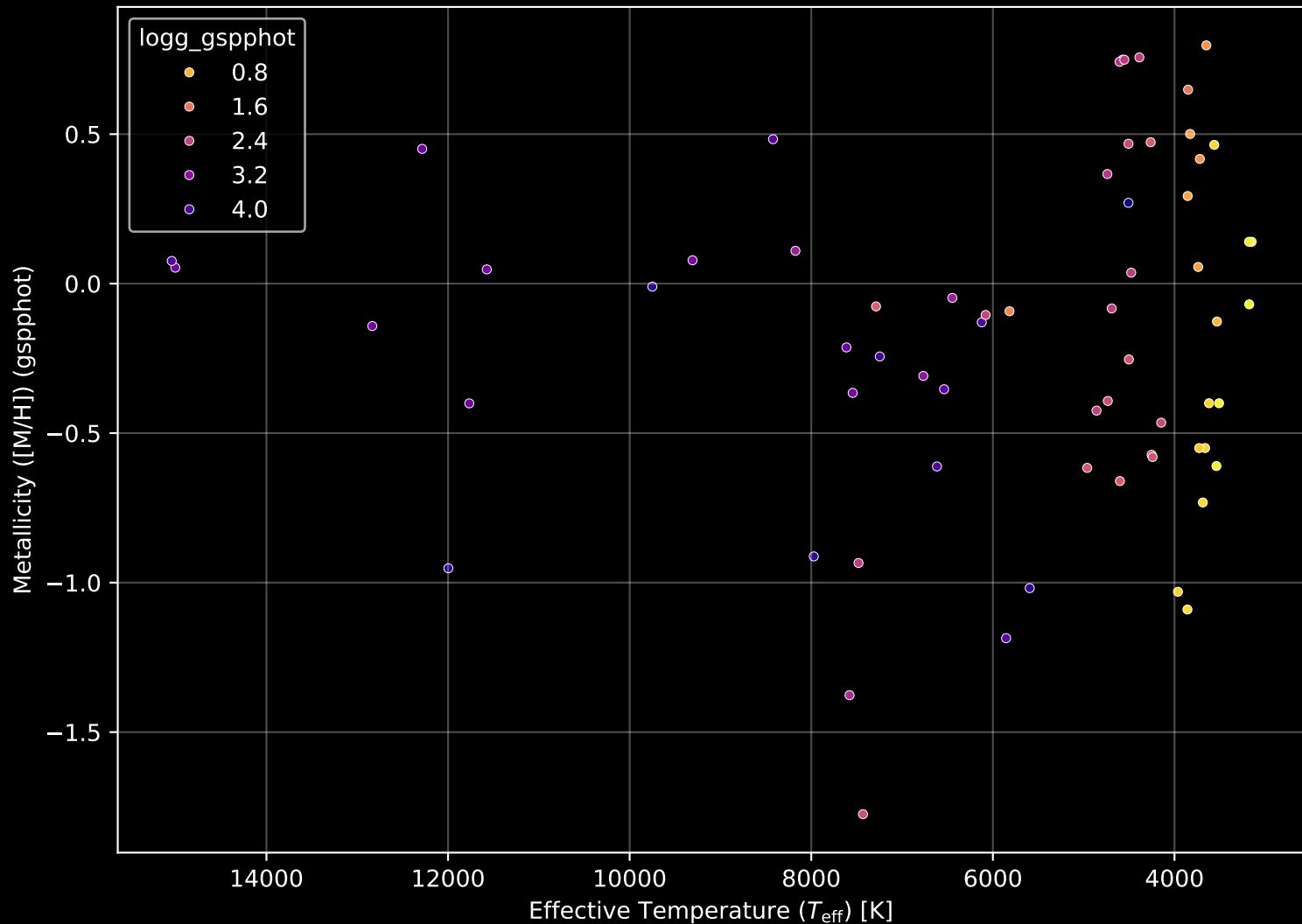
APOGEE DR17 Field: [359+01] Stellar Population Parameters (n= 65)
