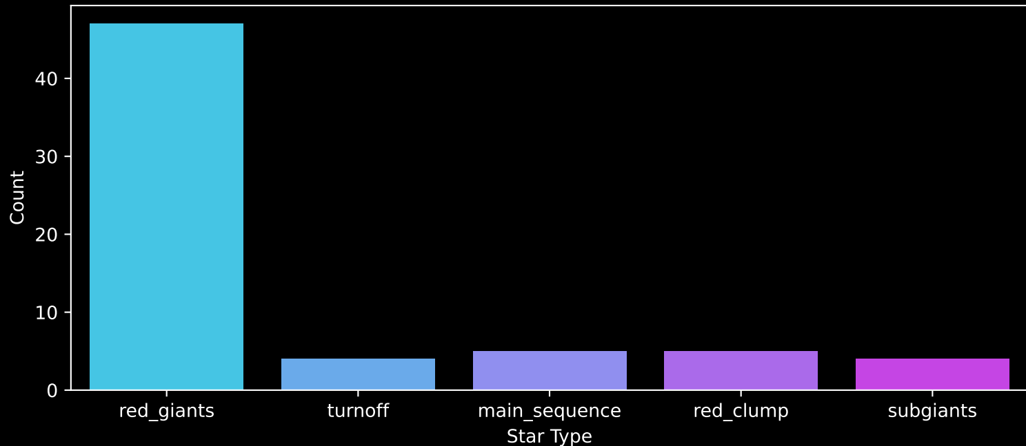
APOGEE DR17 Field: [359+01] Count plot of Star Type
