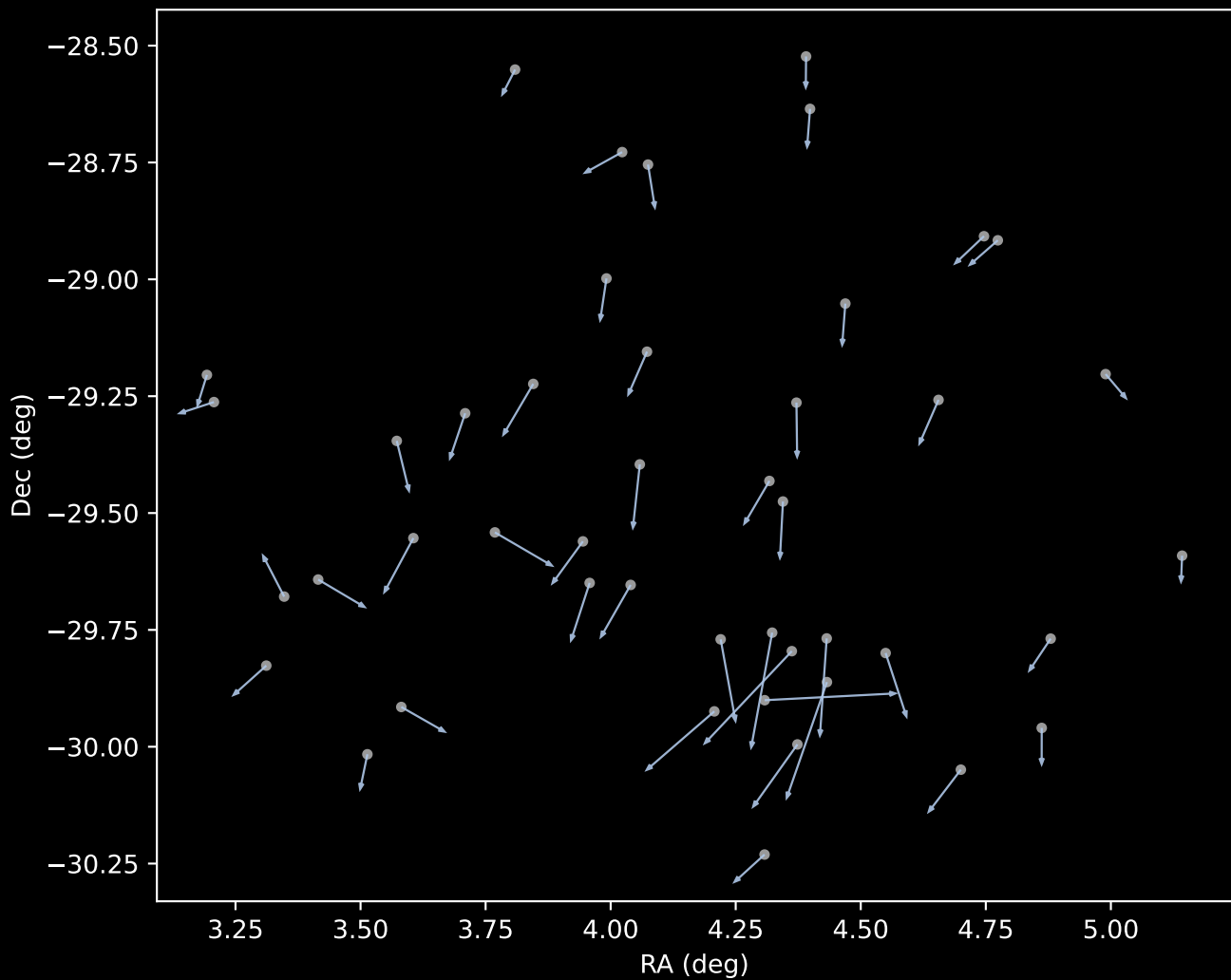
APOGEE DR17 Cluster 1 Proper Motion Vectors (n=45)
