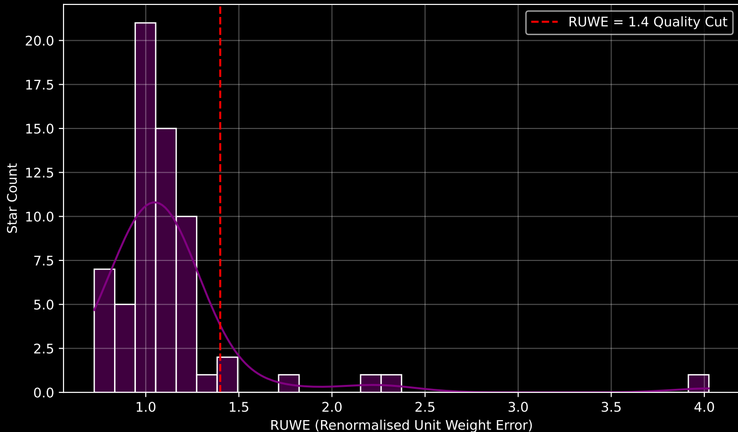
GAPOGEE DR17 Field [359+01] RUWE Distribution (n= 65)
