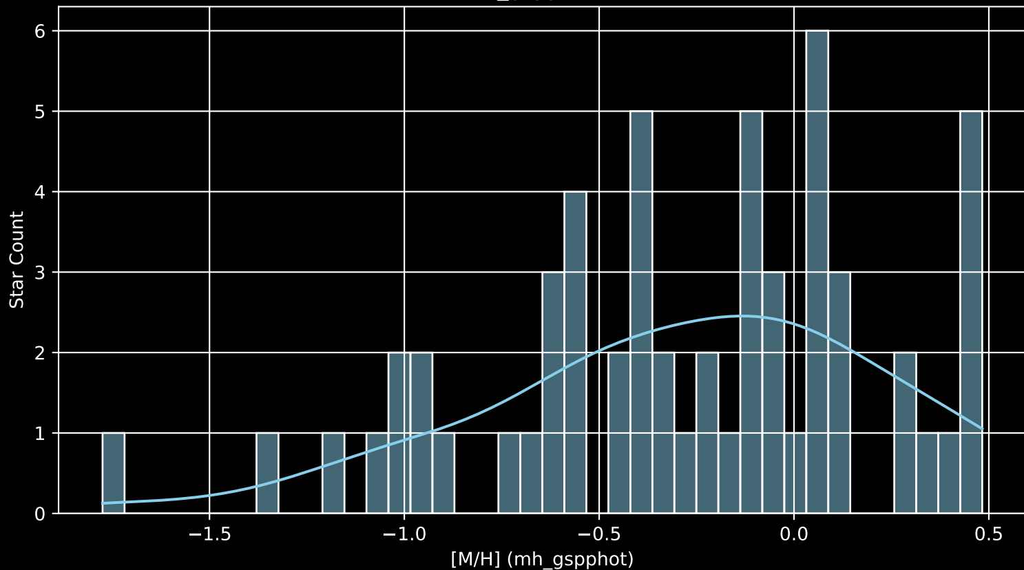
APOGEE DR17 Field: [359+01 [M/H] (mh_gspphot) (n= 58)
