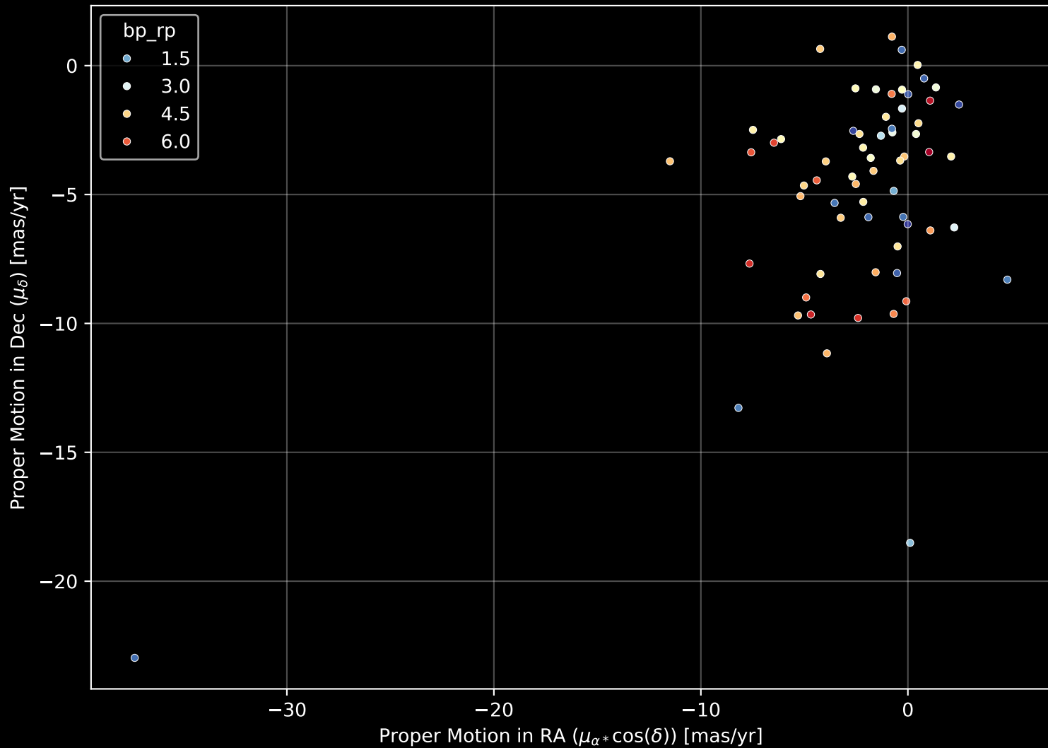
APOGEE DR17 Field: [359+01] Proper Motion Diagram (n= 65)
